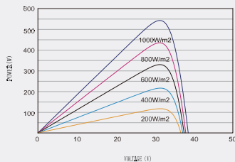
P-V CURVES OF PV MODULE (560W)
